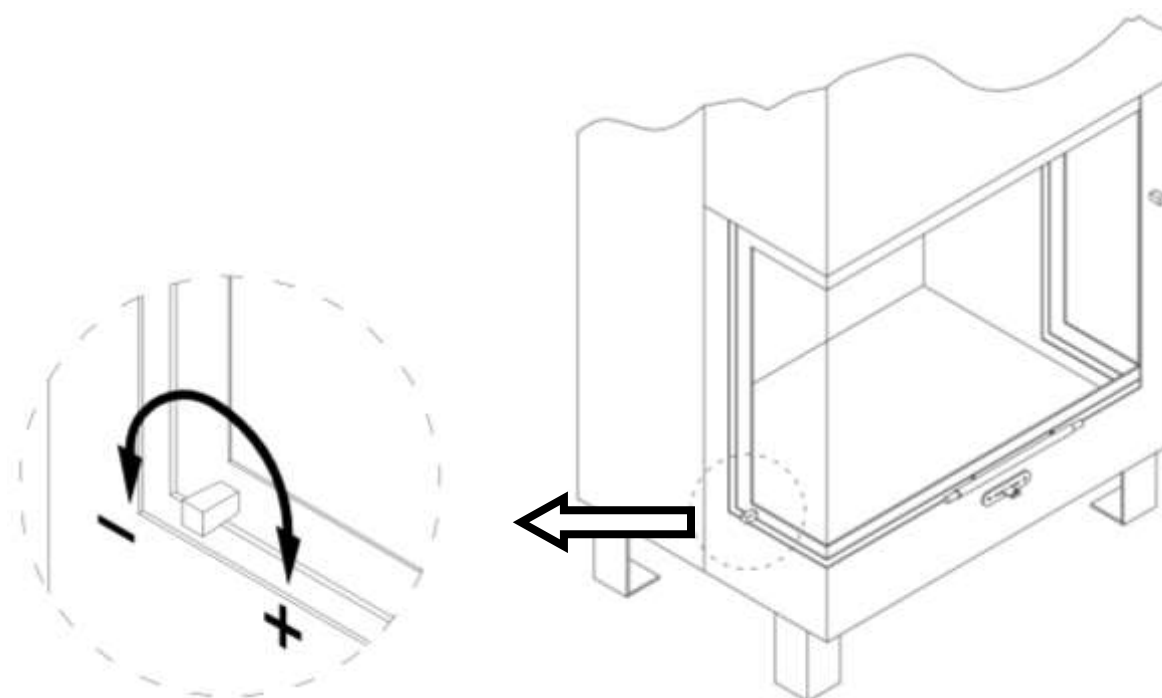
Figure 3: Typical ECO TYPE appliance door frame control
